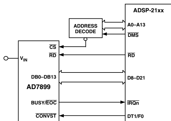
Figure 14. AD7899-ADSP-21xx Interface
